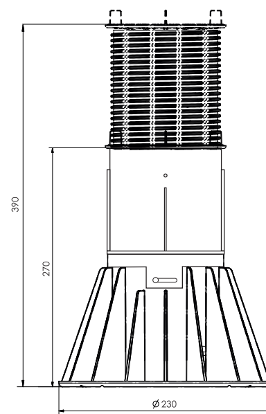
150-270 MM+120 MM ADAPTER
